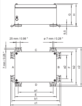
Dimensional Drawing (All Dimensions in mm) - Subject to Alterations
